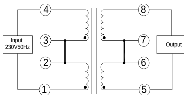
Series Circuit
