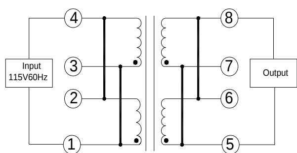
Parallel Circuit
