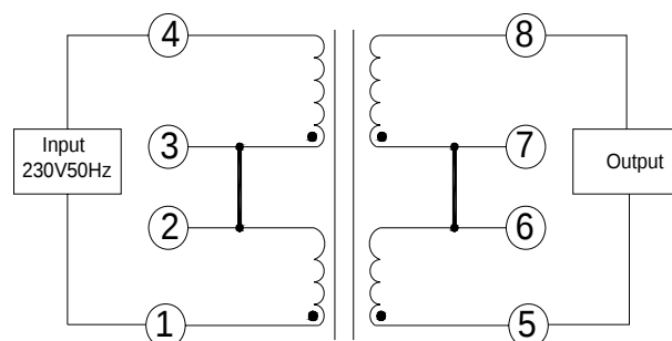
Series Circuit
