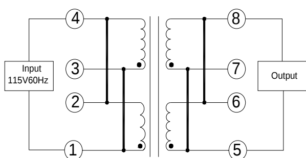
Parallel Circuit
